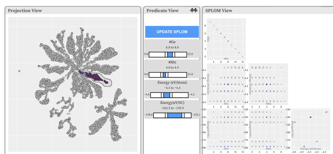
Fig. 8: UI of DimBridge with cluster selected, showing the division of points into clean groups in the SPLOM. This indicates to our collaborator the strong influence Mn has on the clustering of data.
