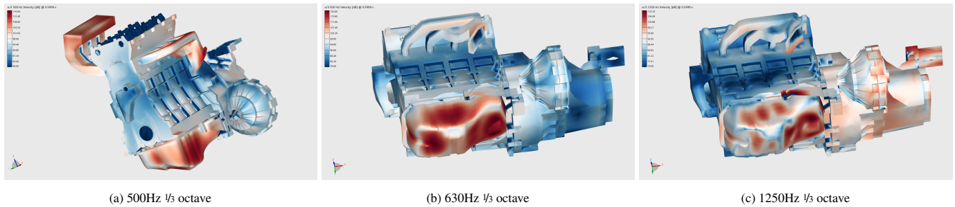
Fig. 12: Velocity levels at the other three critical \frac{1}{3} octaves.
