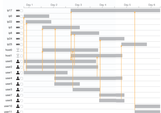
Fig. 3. An anonymized incident report of a red team event. The top visualization shows the unsummarized report, and the bottom shows a summary generated with threshold t = 0.6 .
